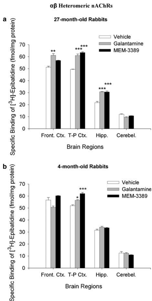
Figure 4 Effect of galantamine and MEM-3389 on expression of \alpha 4\beta 2 nAChRs in four brain regions of (a) 27- and (b) 4-month-old rabbits. B_{\text{max}} values for [^3\text{H}]\text{Epi} binding for \alpha 4\beta 2 nAChRs were determined for frontal cortex, temporal-parietal cortex (T-P cortex), hippocampus, and cerebellum. Each bar represents the mean B_{\text{max}} value from three independent experiments for galantamine, MEM-3389, and vehicle. Vehicle data are also shown in Figure 2. Error bars are SEM. * p < 0.05 ; ** p < 0.01 ; *** p < 0.001 .
